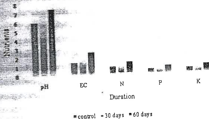
Graph 1: Influence of vermicomposting duration on nutrient content of vermicompost.
