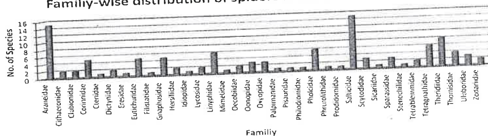
Family-wise distribution of spiders in Lonar Crater Sanctuary
