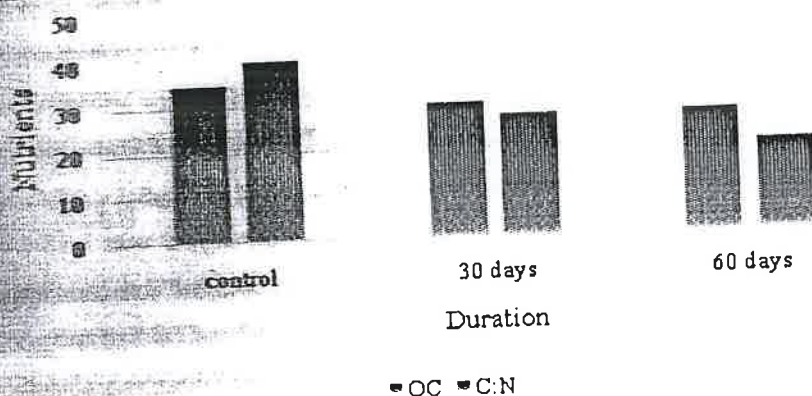
Graph 2: Influence of vermicomposting duration on nutrient content of vermicompost.
