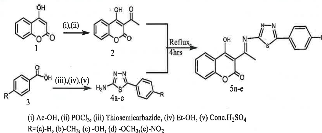
Fig.1: Reaction Scheme for synthesis of Novel Schiff's Bases (5a-5e)
