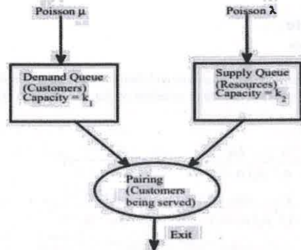
Figure 3: Double ended queue model
