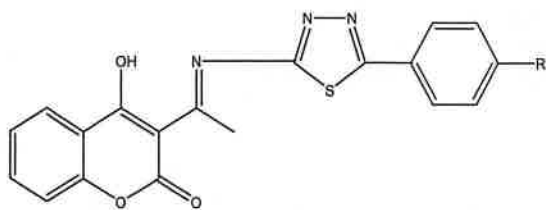
Fig. 1 (Molecular formula C 19 H 12 O 3 N 3 SR)
