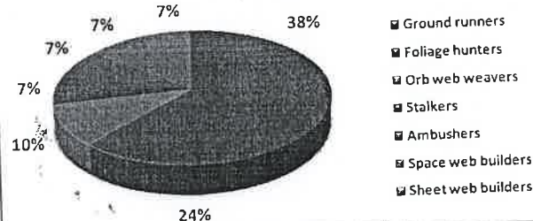
Guid Structure of Spiders collected from Lonar Crater Sanctuary
