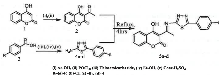
Fig.1: Reaction Scheme for synthesis of Novel Schiff's Bases(SB 5a-d)
